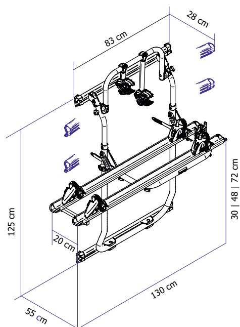
Thule Elite Van XT - Anodised/Black Ducato, Jumper, Boxer ≥ 2007 (art. 81092.95)
