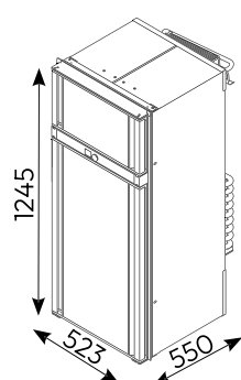
DOMETIC RMD 10.5T
