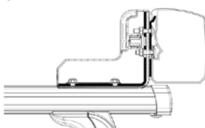
Kit staffe Thule 3200 - Roof Rack
