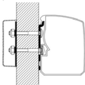
Kit staffe Thule 3200 - Flat Wall
