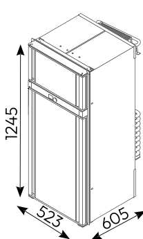
DOMETIC RMD 10.5XP
