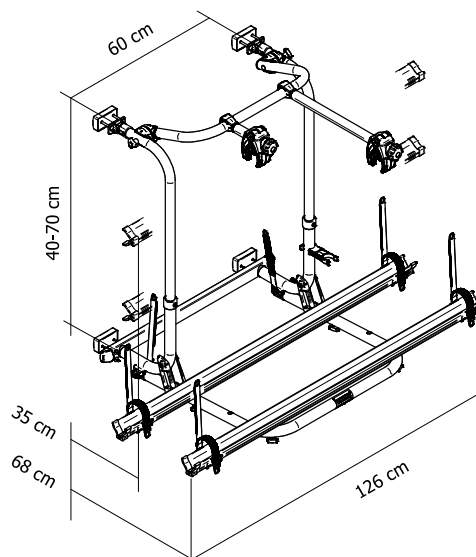
Thule Sport G2 - Short
